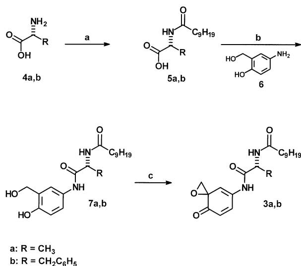
Scheme 1. Synthesis of the scyphostatin analogues 3a,b : (a) H 2 O, THF, Na 2 CO 3 , 18 h, rt, 58%/63%; (b) DCC, HOBT, DMF, 18 h, 26%/39%; (c) NaIO 4 , MeOH/H 2 O, 3 h, rt, 26%/21%.
